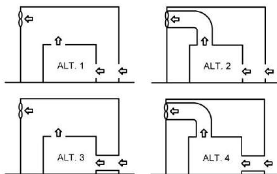
Ventilation proposals (2)
